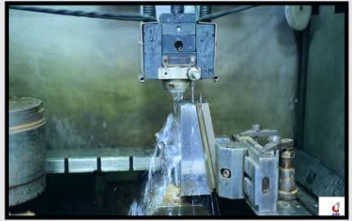
wire-cut Machine
